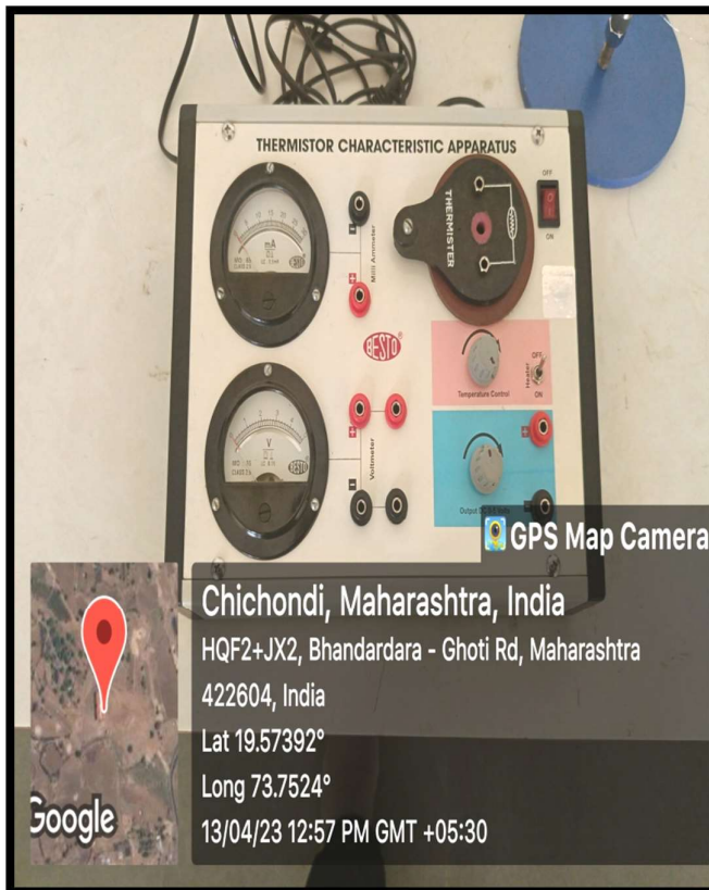
THERMISTOR CHARACTERISTIC
